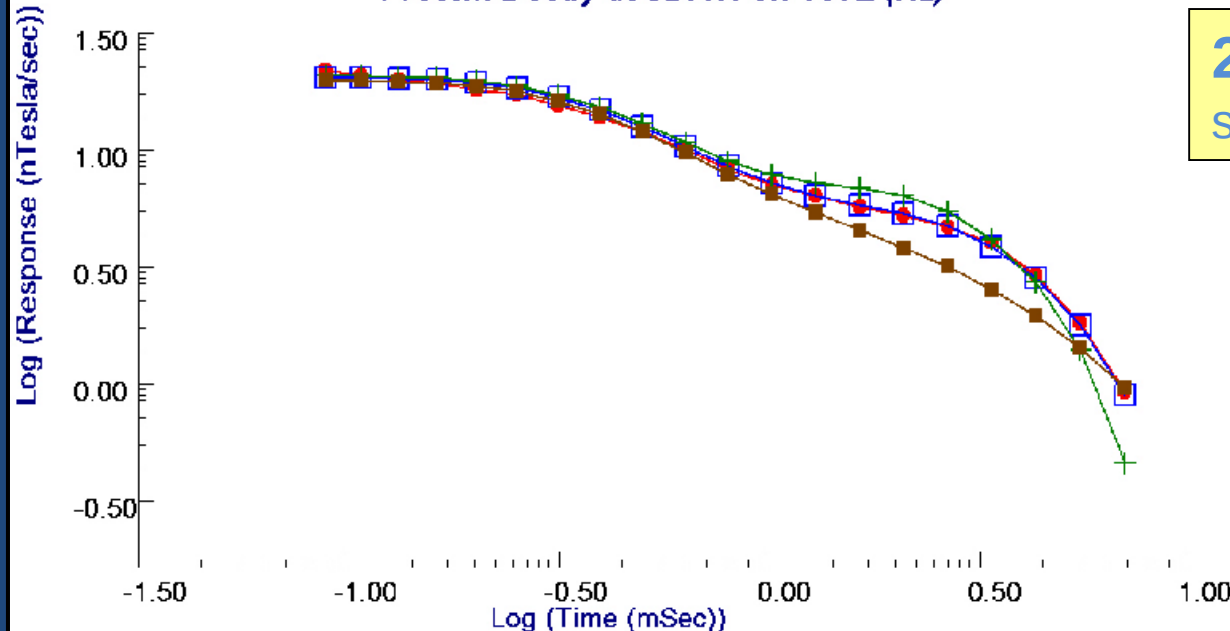
Protem Decay at 3200N on 650E (Hz)
