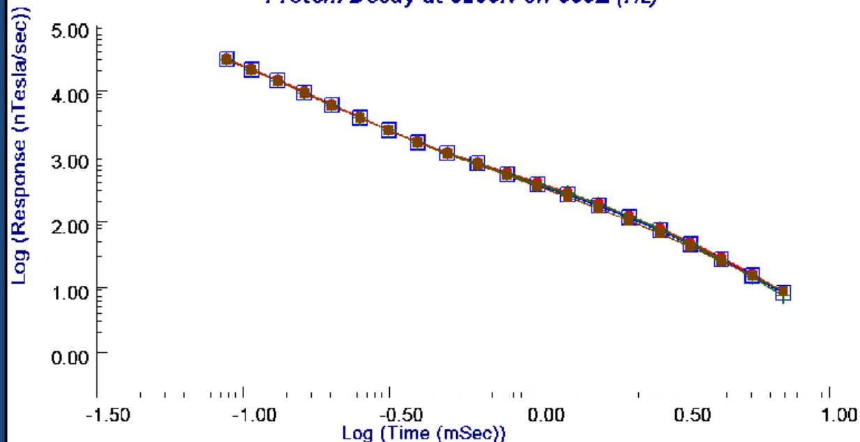
Protem Decay at 5200N on 650E (Hz)
